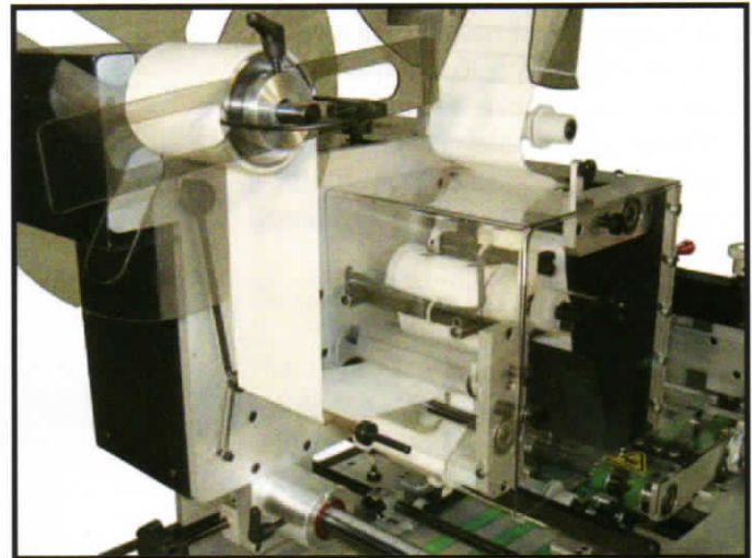
Run 3" wide labels on the standard KR 535. Even wider labels are possible using the optional 5" wide label kit.
